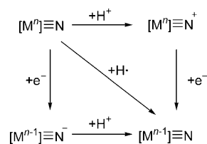
Scheme 1. Thermodynamic cycle for the formation of [M (n-1) ]=NH from [M n ]=N. Concerted HAT follows the diagonal pathway, while stepwise proton and electron transfers follow the horizontal and vertical pathways. [M] represents a metal center and its ancillary ligands.
