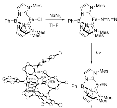
Scheme 2. Synthesis of [PhB(MesIm) 3 Fe≡N] ( 1 ; Mes = 2,4,6-trimethylphenyl). Inset: X-ray crystal structure of 1 ; solvent molecules and hydrogen atoms are omitted for clarity.
